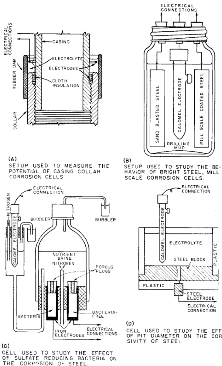
FIG. 9—VARIOUS LABORATORY SET-UPS USED TO STUDY THE PROCESSES OF EXTERNAL CASING CORROSION.
