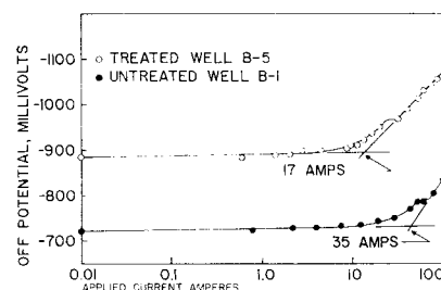
FIG. 11—EFFECT OF HYDRAZINE ON CATHODIC-PROTECTION CURRENT REQUIREMENTS.
