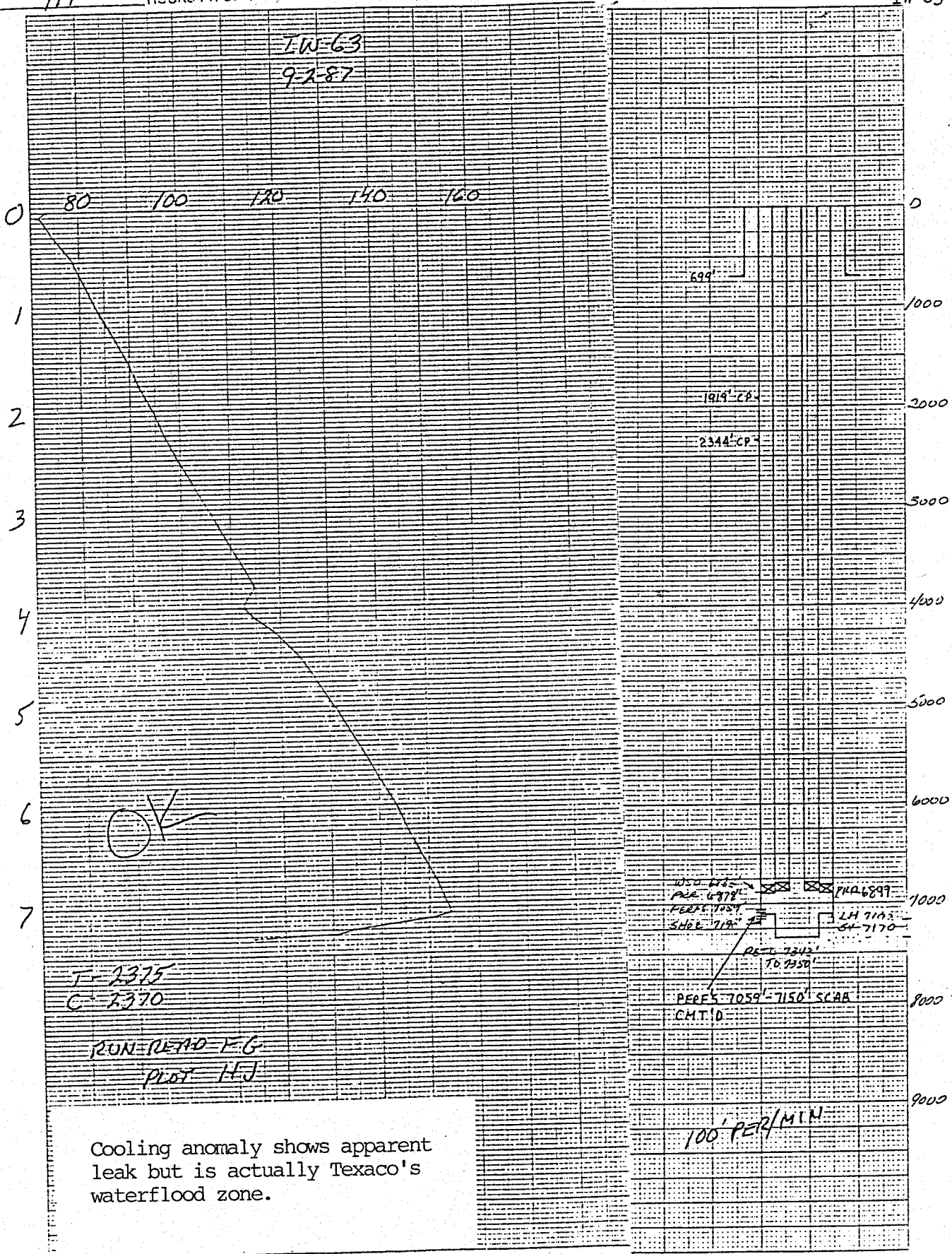
FIGURE 13. TEMPERATURE SURVEY
