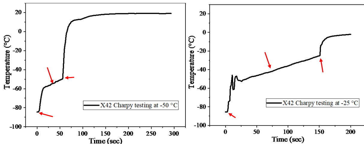
Figure 104: Temperature Profiles in the Low-Temperature Charpy Testing on X42
