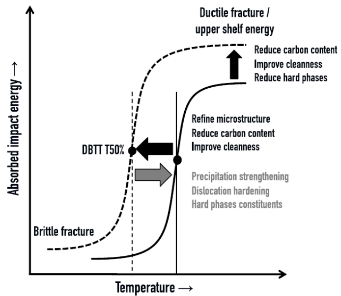
Figure 78: Ductile to Brittle Transition
