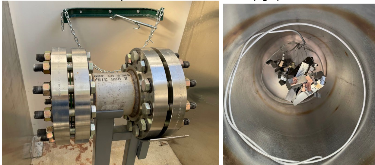
Figure 83: View of Test Chamber with Heating Element and Thermal Insulation
